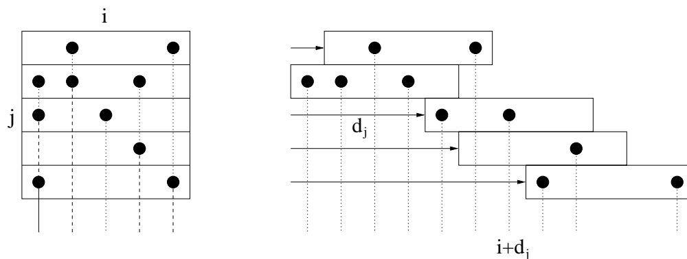
Figure 1: Tarjan-Yao displacement scheme
